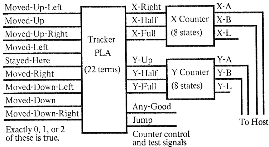
Figure 11. Tracking Spots by Comparing Images
