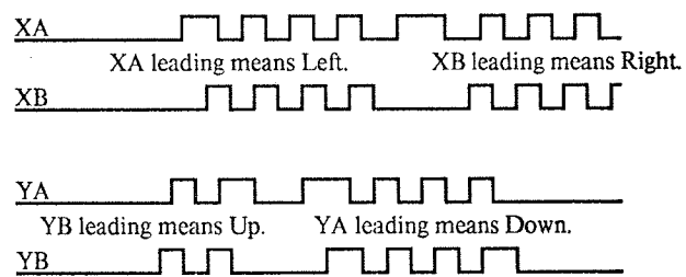
Figure 2. Quadrature Encoding of Pointer Motion on a Bitmap Display System.
