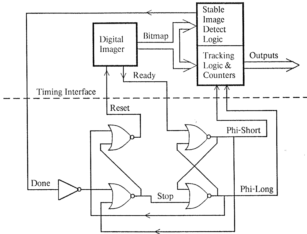
Figure 9. Imager and Logic tied together by Self-timed Clock Circuit, with timing waveform diagram.
