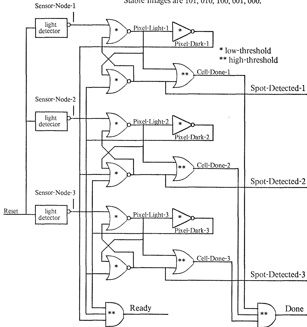
Figure 15. Three-pixel Dark-spot Sensor Example, with nearest-neighbor inhibition. Stable Images are 101, 010, 100, 001, 000.
